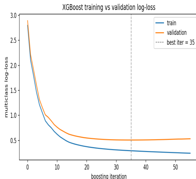
Figure 4.5. XGBoost training vs validation log-loss.
