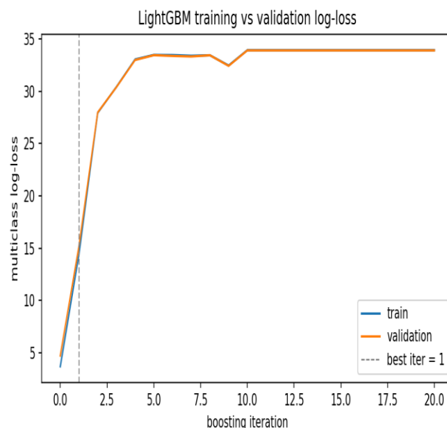
Figure 4.6. LightGBM training vs validation log-loss.
