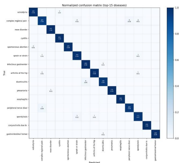
Figure 4.4. Multilayer perceptron normalised confusion matrix (top-15 diseases).
