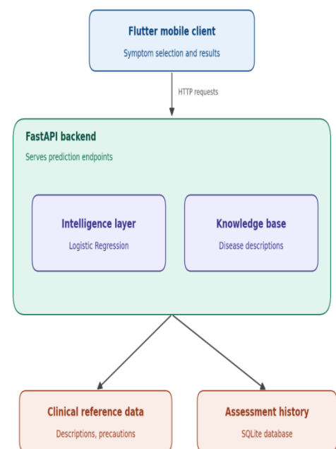
Figure 3.1. Smart Health Assistant three-tier system architecture.
