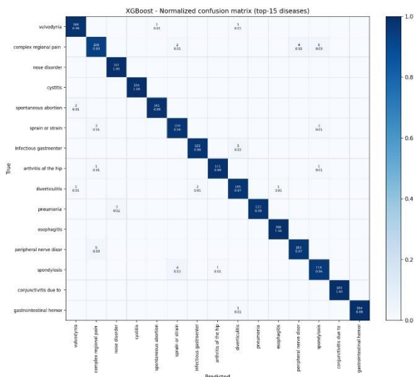
Figure 4.1. XGBoost normalised confusion matrix (top-15 diseases).
