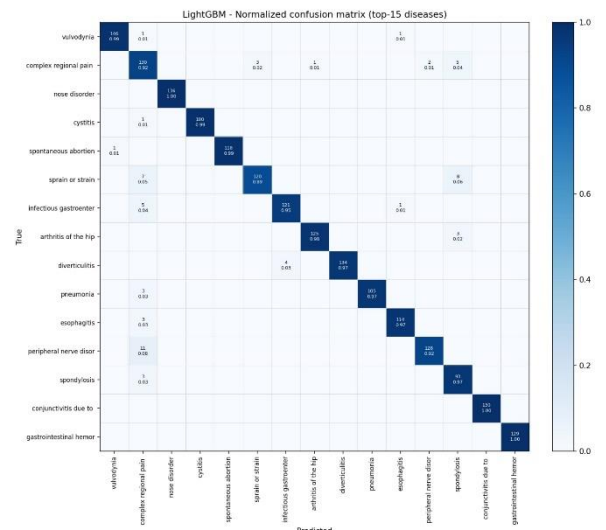
Figure 4.2. LightGBM normalised confusion matrix (top-15 diseases).
