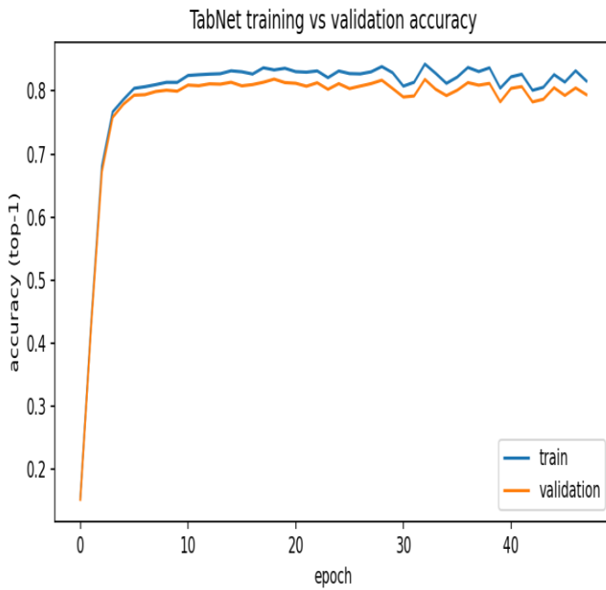
Figure 4.7. TabNet training vs validation accuracy.
